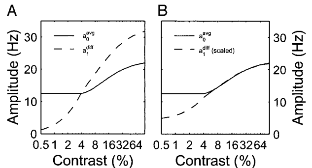
FIG. 3. The condition for contrast invariance is satisfied above 5% Contrast. A: a_0^{\text{avg}} and a_1^{\text{diff}} as functions of contrast for the linear rectified LGN responses to drifting sinusoidal gratings shown in Fig. 1. B: a_0^{\text{avg}}(C) and a rescaled and offset version of a_1^{\text{diff}}(C) [ 0.56 + 4.16a_1^{\text{diff}}(C) - determined by a linear regression calculated at 50 contrasts equally spaced on a log scale between 5 and 100% contrast].
