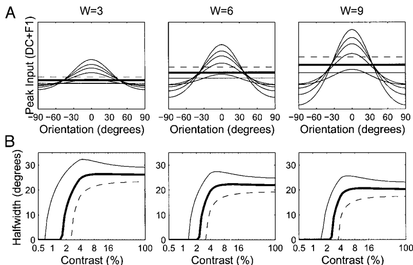
FIG. 4. Dependence of contrast invariance on the 2 model parameters, w and \psi^{eff} , using the linear rectified model of response to drifting sinusoidal gratings of Fig. 1. A: peak input as a function of orientation at 5 different contrasts (2, 4, 8, 16, and 64%) for 3 different levels of inhibition (left: w = 3 ; middle: w = 6 ; right: w = 9 ). All plots are shown with background level of input subtracted. Units chosen so that the modulation of the excitatory input for an optimal stimulus has unit magnitude [ F1_{max}(100)h(0) = 1 ]. The 3 horizontal lines show 3 possible levels of effective threshold \psi^{eff} . The thick line represents the optimal threshold as defined by linear regression as in Fig. 3B. The thin and dashed lines deviate from this optimal by \pm 0.1(1 + w)F1_{max}(100) , i.e., \pm 10\% of the total input modulation at 100% contrast. B: orientation tuning halfwidth as a function of contrast for the 3 levels of effective threshold shown in A. Peak inputs were calculated using Eq. 10 with \phi_{stim} = 1 . Halfwidths were calculated from tuning curves constructed by integrating Eq. 11 over a complete cycle.
