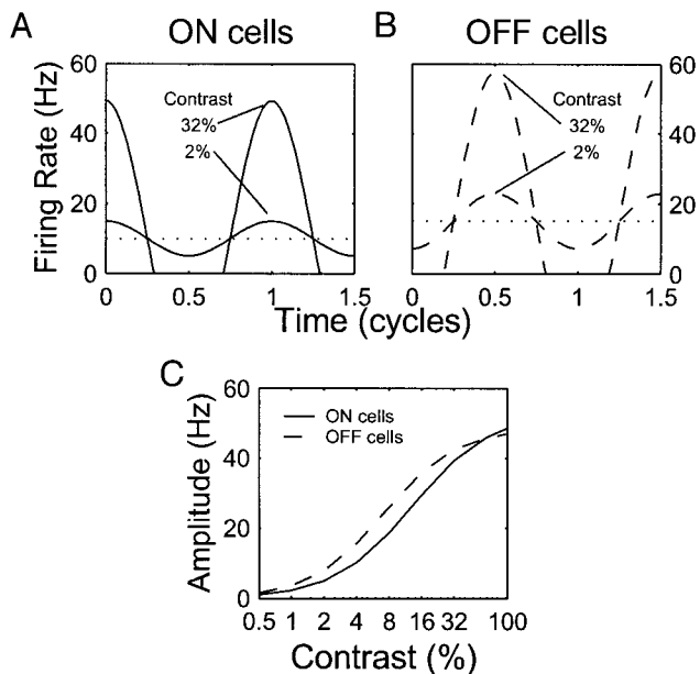
FIG. 1. Linear rectified model of lateral geniculus (LGN) response to drifting sinusoidal gratings. A and B : response of ON and OFF cells to drifting sinusoidal gratings of 2 and 32% contrast. C : modulation amplitude as a function of contrast for ON and OFF cells (computed from F_1 of spiking response from Cheng et al. 1995, assuming background firing rates of 10 and 15 Hz, respectively, and a linear rectified model of LGN response; see METHODS in Troyer et al. 1998).
