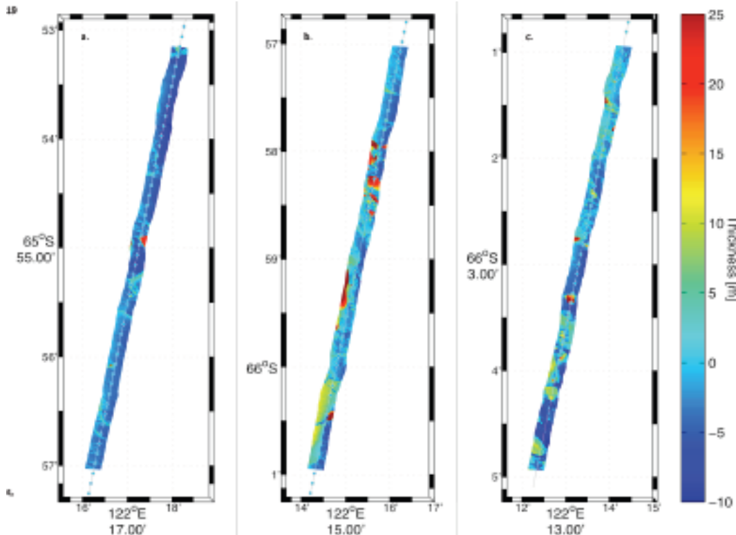
Figure 3: Three legs of the aerial survey underlying ICESat track 0466. Each leg consists of 4000 scanner lines (approx. 7.3 km flight track) and are consecutive from North to South (a to c). Colour-coded are laser scanner ice thickness estimates following equations 1 and 2. Also shown with colour filled circles are ICESat sea ice thickness estimates using the same colour scale.
