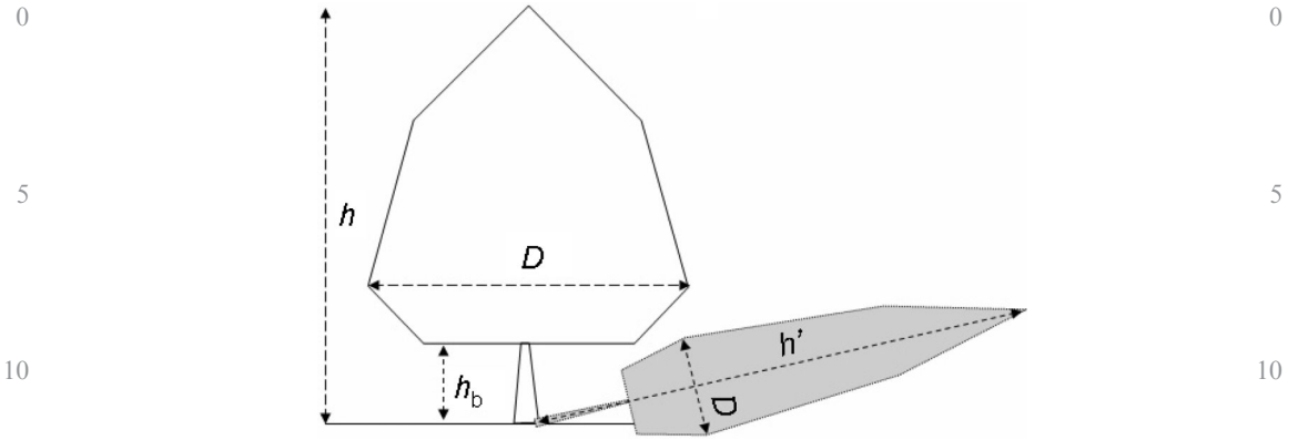
Figure 3. The tree shadow caused by the oblique solar position.
