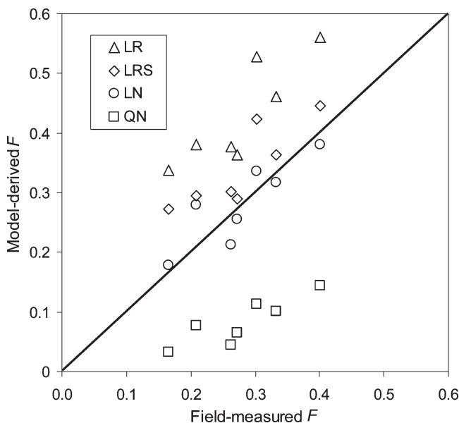
Figure 5. Comparison of model-estimated F and field-measured F within the seven sample cells in the woodland biomass zone. LR, linear reflectance model; LRS, linear reflectance model with shadow correction; LN, linear NDVI model; QN, quadratic NDVI model.
